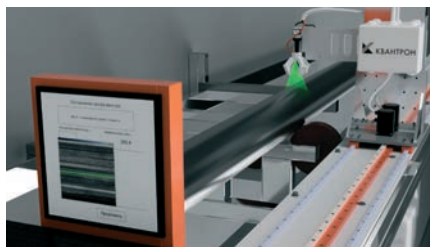
Slotted Filter Inspection Machine
